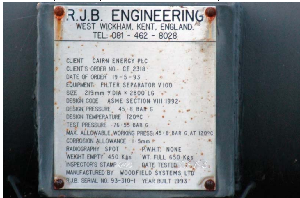
Filter separator specification plate with no evidence of re-inspection dates
