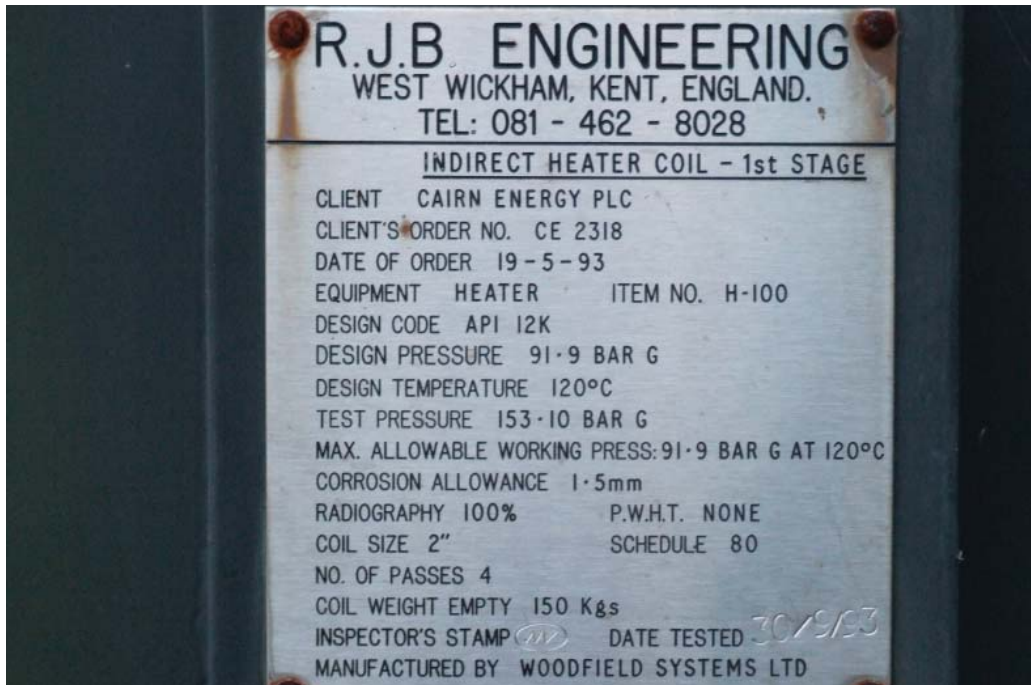
Heater coil specification plate with no evidence of re-inspection dates
